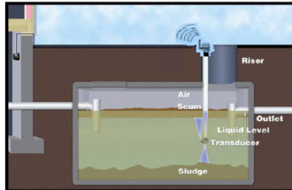
Diagram of 1000 Gallon Grease Trap
